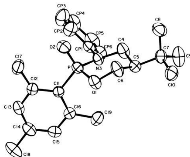
Figure 2. ORTEP plot for trans -12. 5
